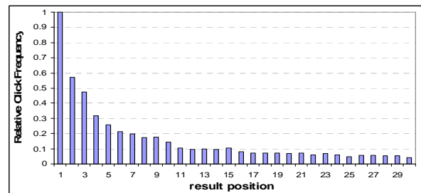
Figure 3.1: Relative click frequency for top 30 result positions over 3,500 queries and 120,000 searches.
