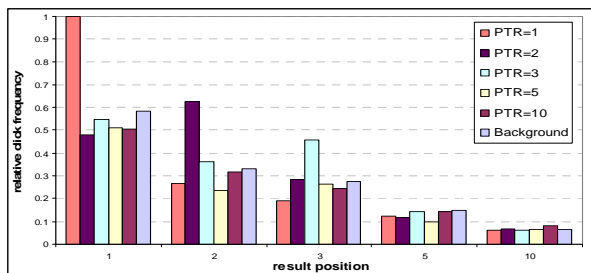
Figure 3.2: Relative click frequency for queries with varying PTR (Position of Top Relevant document).
